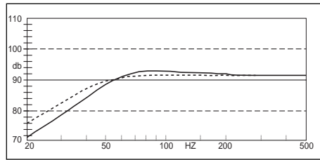
sealedbox - 30 l ... 75 l
